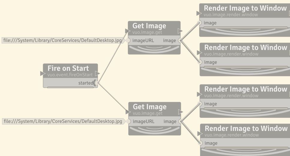
Multiple data-and-event and event-only cables can be connected to an output port.
