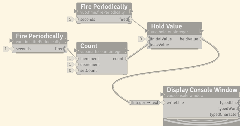
A composition, Count and Hold, showing nodes executing at different rates
