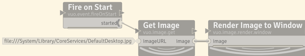
A sample composition, DisplayImage.vuo, with three nodes and two cables
