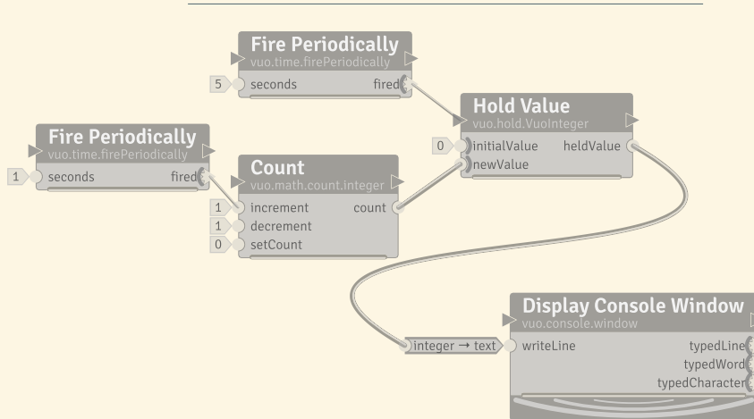
A sample composition, CountandHold.vuo, using a Hold Value node
