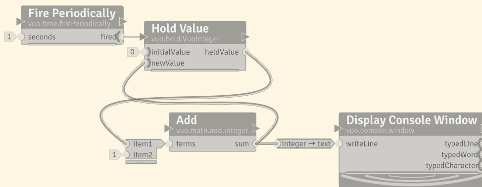
A composition, CountWithFeedback.vuo, showing a feedback loop .
