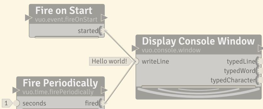
Multiple event-only cables, but only one data-and-event cable, can be connected to an input port.
