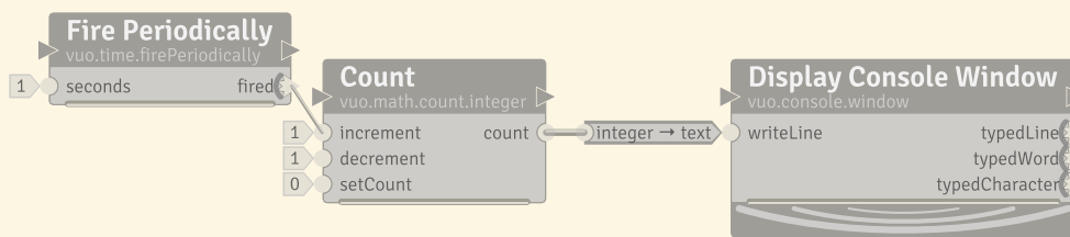
The sample composition, Count.vuo
