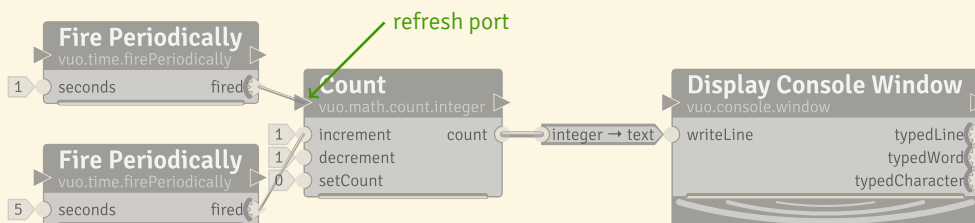
A sample composition, CountSometimes.vuo , using a refresh port
