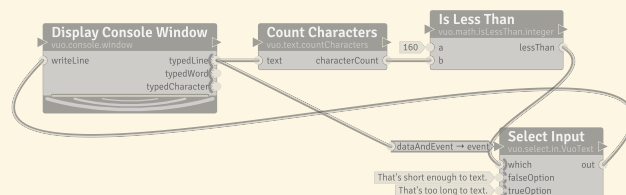
A composition, Check SMS Length, showing a type converter discarding data from an event
