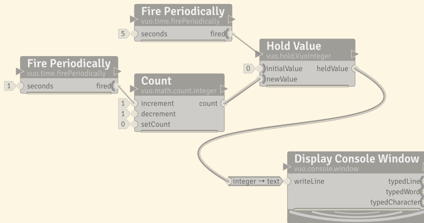
A sample composition, CountandHold.vuo, using a Hold Value node
