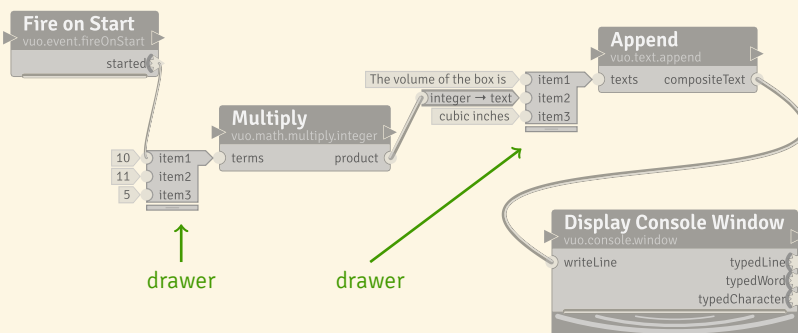
A composition that takes the height, length, and width of a box and calculates its volume
