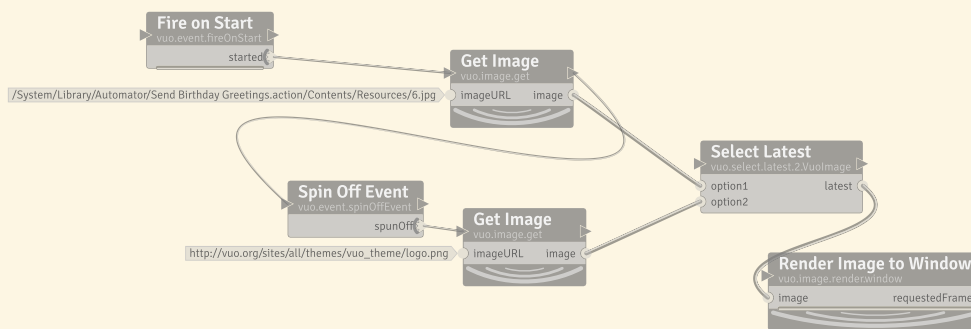
A composition, LoadImagesAsynchronously.vuo, has nodes execute in the background
